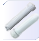
Membrane Vessel for 200 / 700 GPD RO 1812 Ports 1/8" NPT x 1/8" NPT x 1/8" NPT
